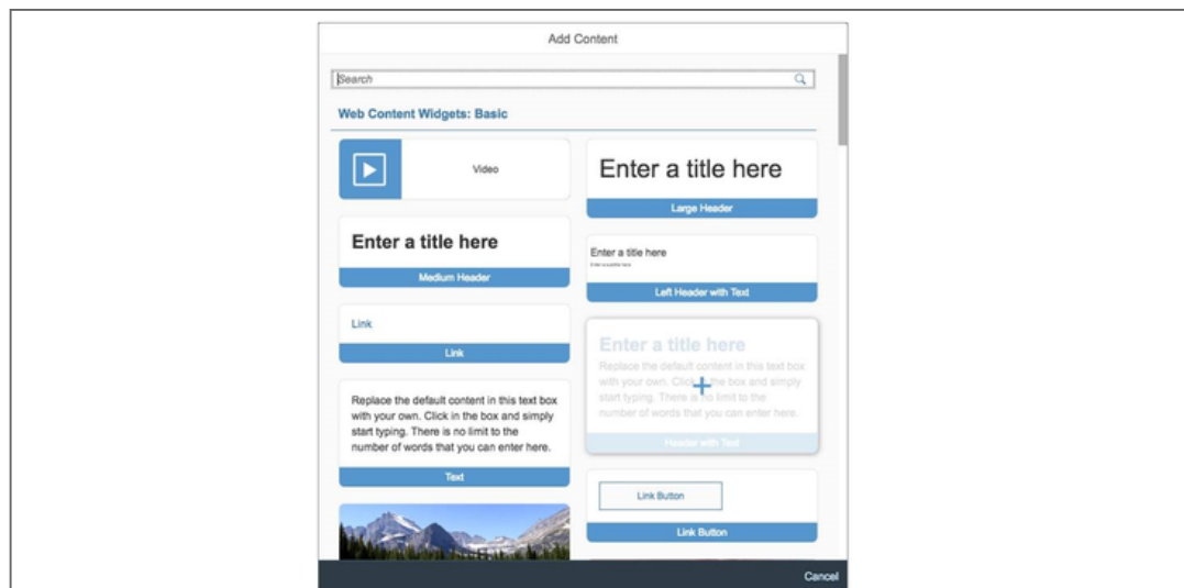
Figure 64: Widgets
