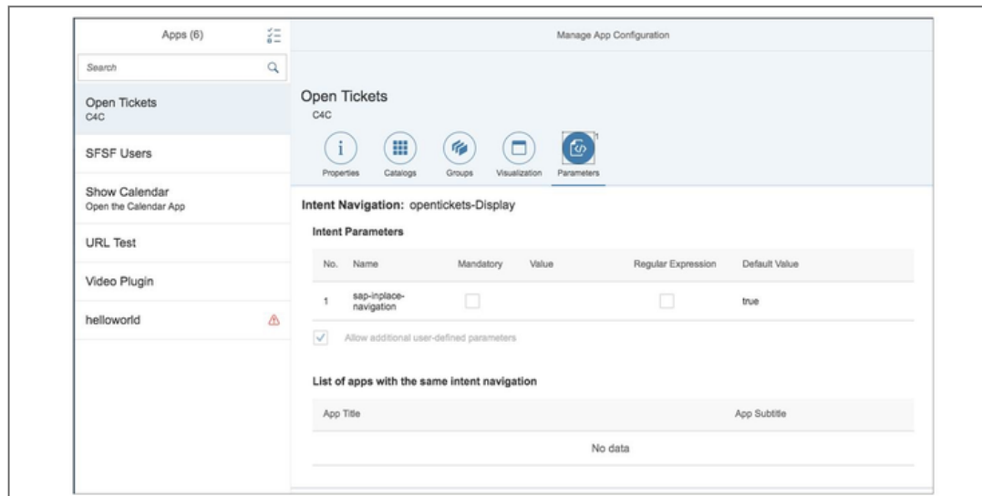
Figure 22: Navigation Parameters
