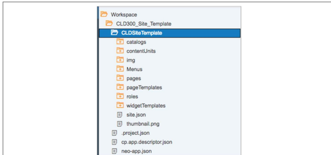
Figure 57: Project Structure
