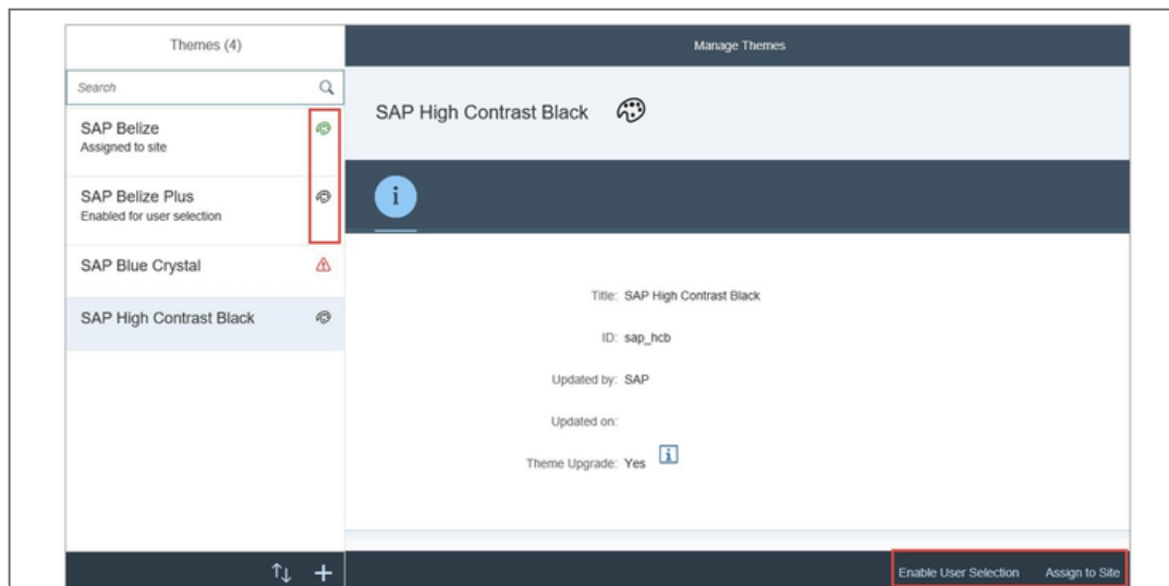
Figure 75: Configuring Themes
