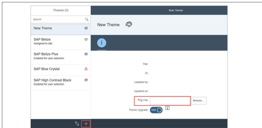
Figure 76: Transporting Themes
