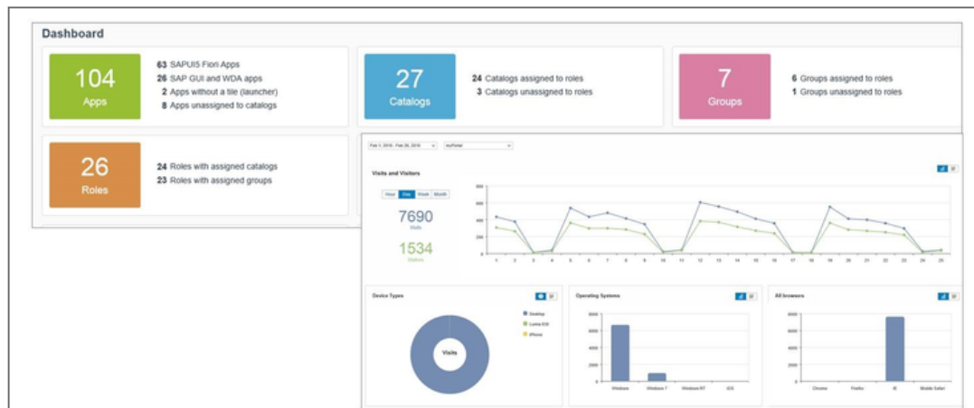
Figure 93: Site Statistics
